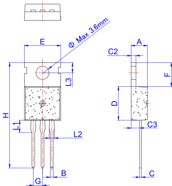
TO-220C
