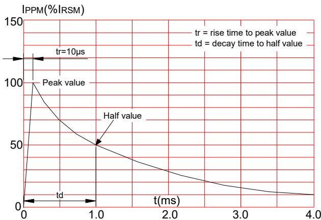
FIG.5: ISO16750 -2 test pulse 5a
