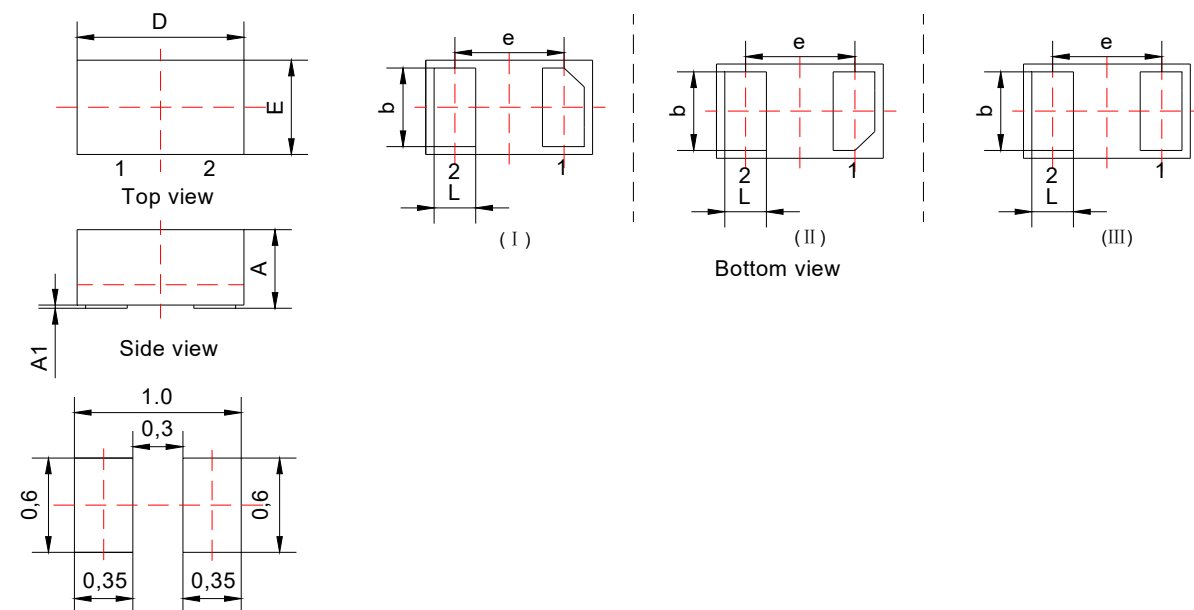
Recommended soldering footprint(mm)
