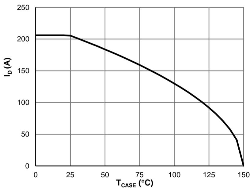
Figure 9: Current De-rating
