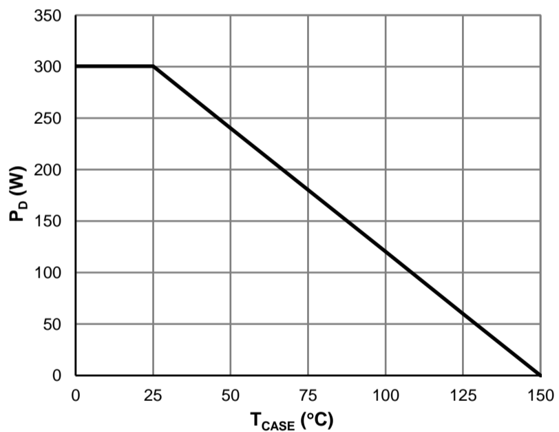
Figure 10: Power De-rating
