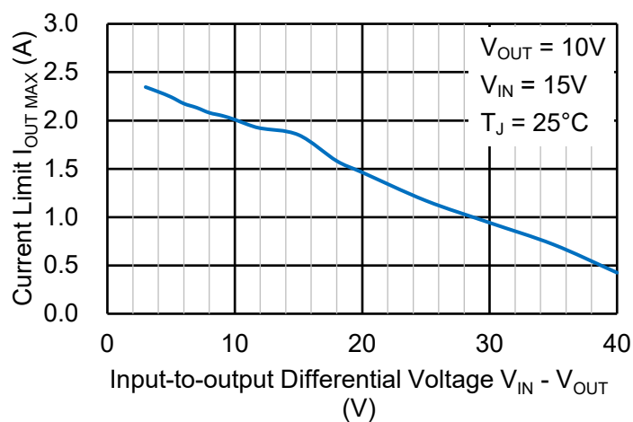
Current Limit
