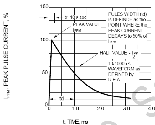
FIG.3 -- PULSE WAVEFORM
