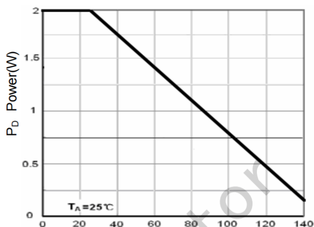
Tj-Junction Temperature(°C)
