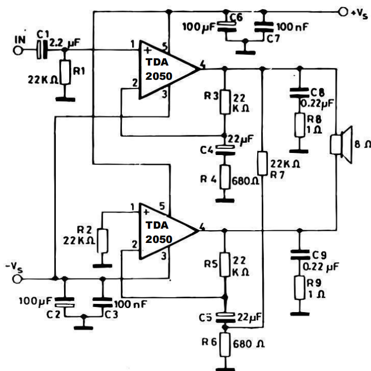
Figure 13 : Bridge Amplifier with Split Power Supply ( P_O = 34\text{W} , V_S = \pm 16\text{V} )
