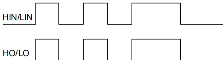
Figure 5. TF2101M Input and output timing waveform
