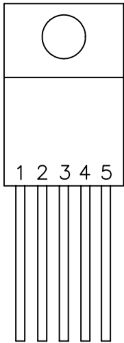
TO-220-5
