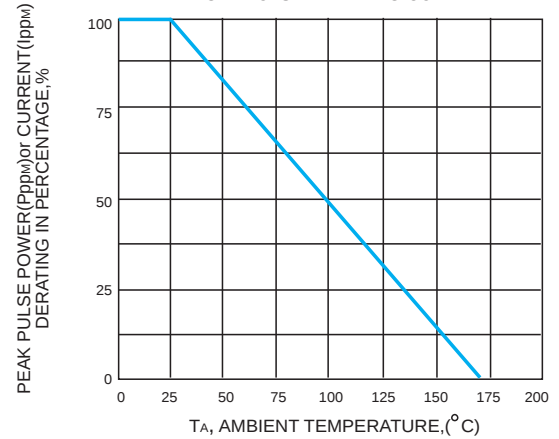
FIG. 2-PULSE DERATING CURVE
