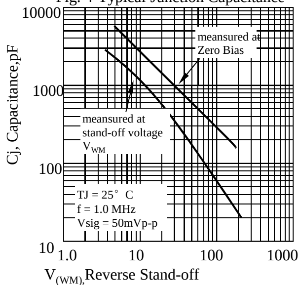
Fig. 4-Typical Junction Capacitance
