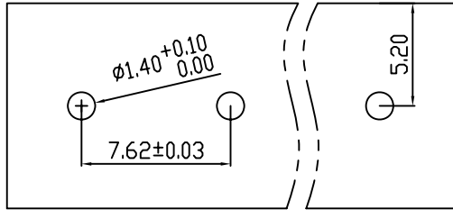
PCB LAYOUT
