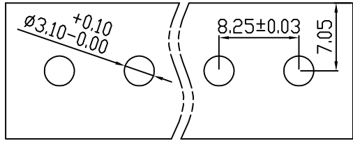
PCB LAYOUT
