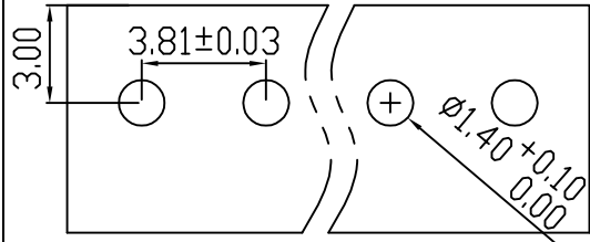
PCB LAYOUT
