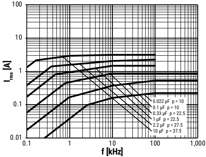
630 VDC/275 VAC
