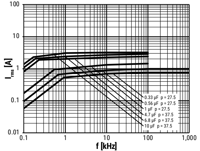
1,000 VDC/275 VAC
