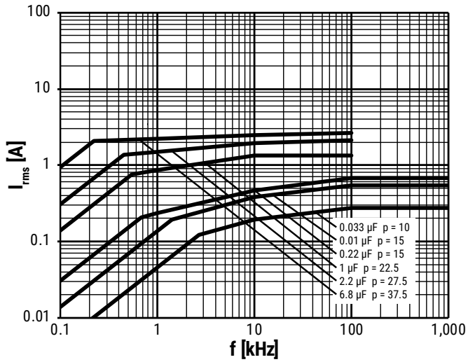
630 VDC/275 VAC
