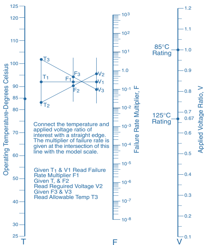
Fig 6 Reliability alignment chart
