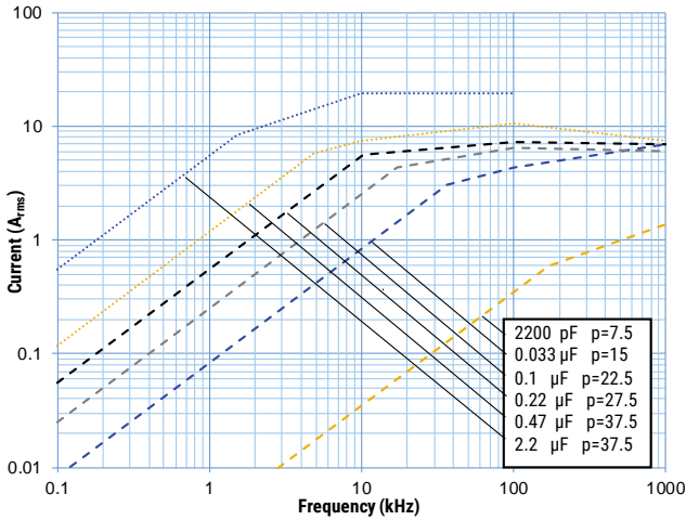
630 VDC/400 VAC
