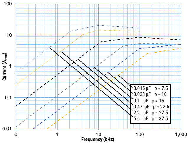
250 Vdc / 180 Vac
