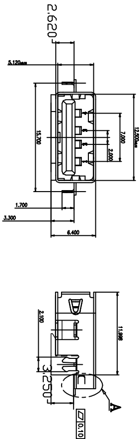
RECOMMENDED P.C.B. PATTERN LAYOUT
