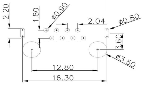
PCB
