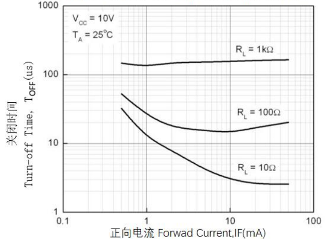
Figure 6. Turn-off Time vs Forward Current
