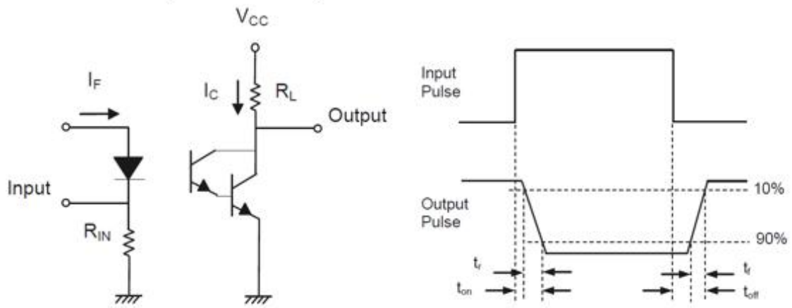
Figure 7. Switching Time Test Circuit &amp; Waveforms
