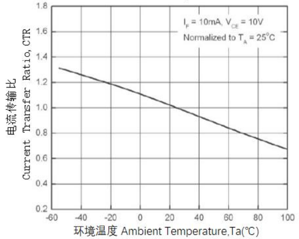
Figure 2. Current Transfer Ratio vs Ambient Temperature
