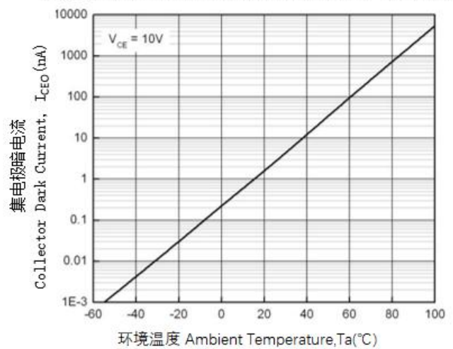
Figure 4. Collector Dark Current vs Ambient Temperature
