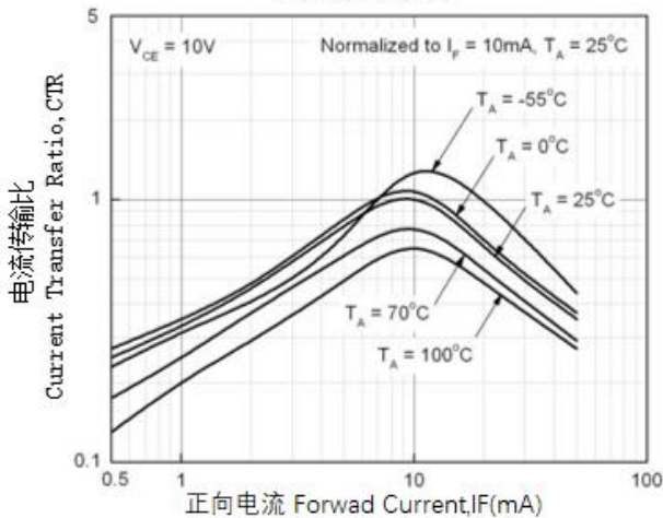
Figure 3. Normalized Current Transfer Ratio vs Forward Current
