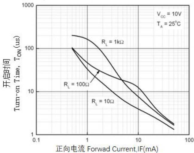
Figure 5. Turn-on Time vs Forward Current
