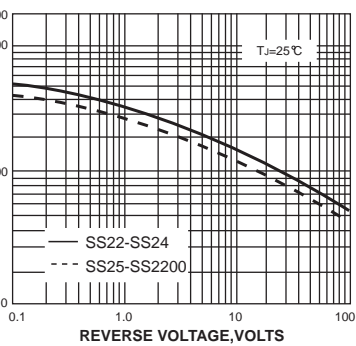
FIG. 5-TYPICAL JUNCTION CAPACITANCE
