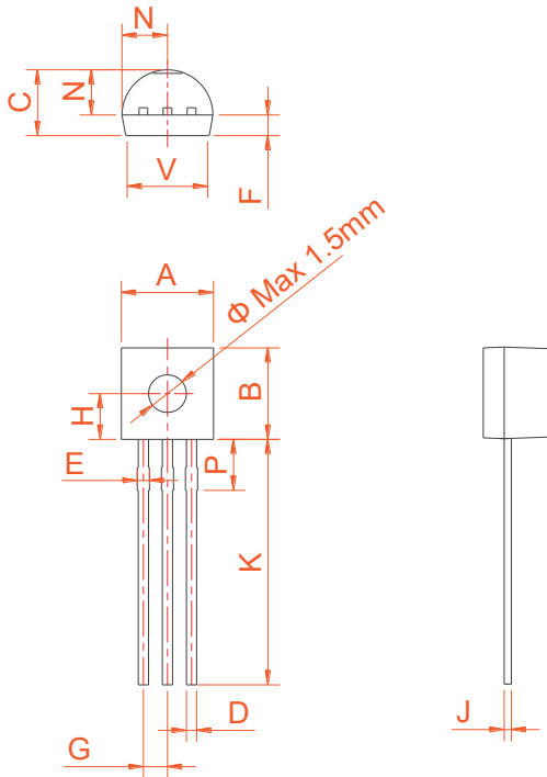
TO-92
