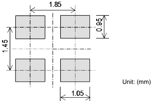
Fig.4 Land pattern
