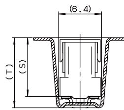
SECT. F-F
