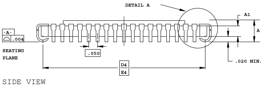
SIDE VIEW
