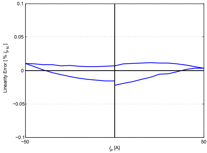
Figure 16: Linearity error
