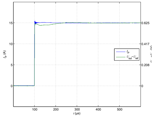
Figure 8: Delay time
