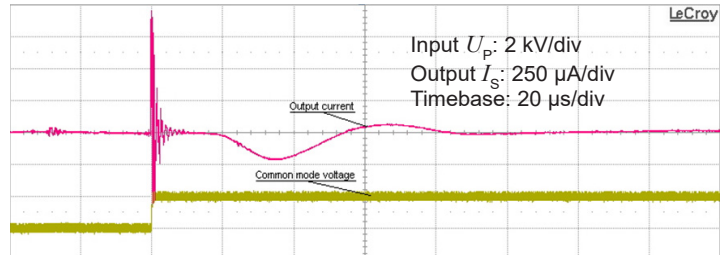
Figure 12: Detail of typical common mode perturbation (150 V step with 6 kV/μs, R_M = 100 \Omega )
