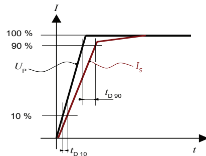
Figure 17: Delay time t_{D90} @ 90 and delay time t_{D10} @ 10
