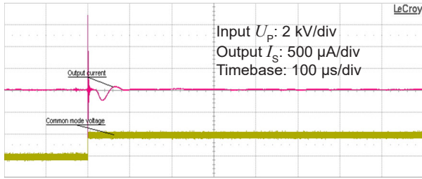
Figure 11: Typical common mode perturbation (150 V step with 6 kV/μs, R_M = 100 \Omega )
