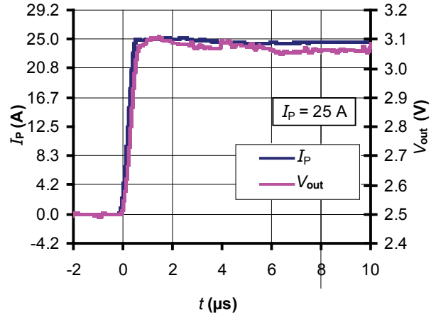
Figure 4: Step response
