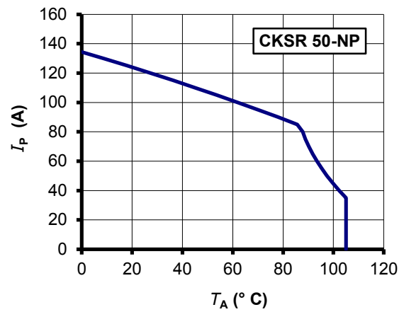
Figure 14: I_P vs T_A for CKSR 50-NP/SP1
