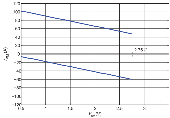
Figure 19: Measuring range versus external V_{ref} LESR 15-NP/SP1
