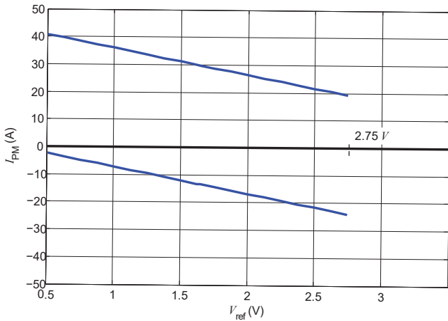
Figure 18: Measuring range versus external V_{ref} LESR 6-NP/SP1
