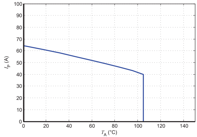
Figure 12: I_p vs T_A for LESR 15-NP/SP1
