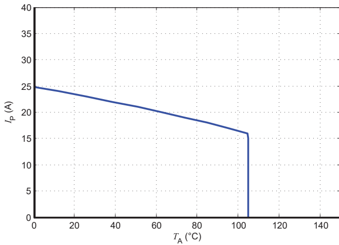
Figure 11: I_p vs T_A for LESR 6-NP/SP1
