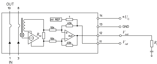
Figure 15: Test connection
