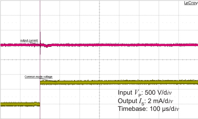
Figure 11: Typical common mode perturbation (750 V step with 6 kV/μs R_M = 100 \Omega )
