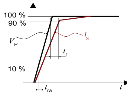
Figure 17: Response time t_r and reaction time t_{ra}
