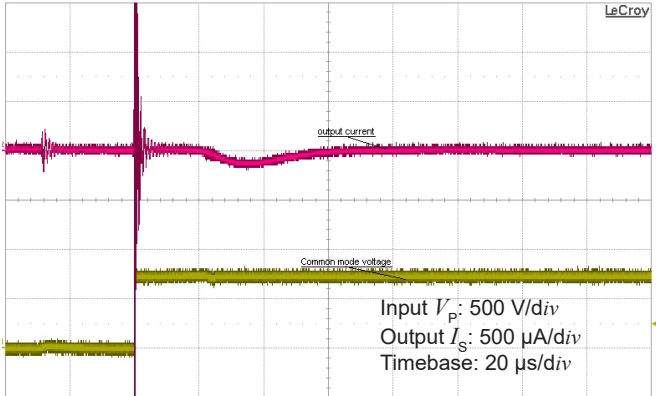
Figure 12: Detail of typical common mode perturbation (750 V step with 6 kV/μs, R_M = 100 \Omega )
