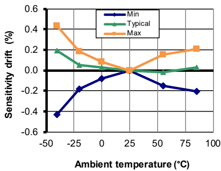
Figure 5: Sensitivity thermal drift
