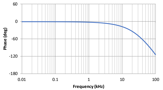
Figure 9: Phase shift function of frequency
