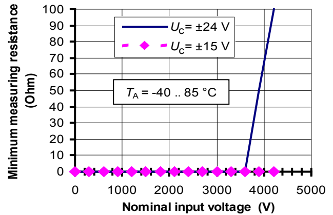
Figure 2: Minimum measuring resistance For T_A under 80 °C, the minimum measuring resistance is 0 Ω whatever U_C
