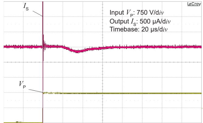
Figure 12: Detail of typical common mode perturbation (1500 V step with 6 kV/μs, R_M = 100 \Omega )
