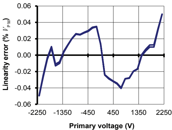
Figure 15: Typical linearity error at 25 °C
