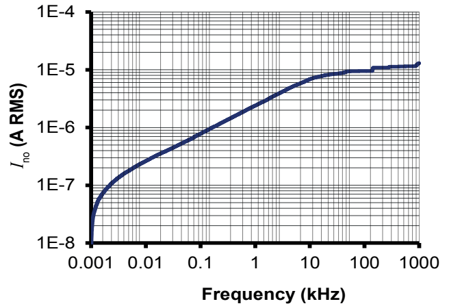
Figure 14: Typical total output RMS noise current with R_M = 50 \Omega ( f_c is upper cut-off frequency of bandpass, low cut off frequency is 1 Hz)
