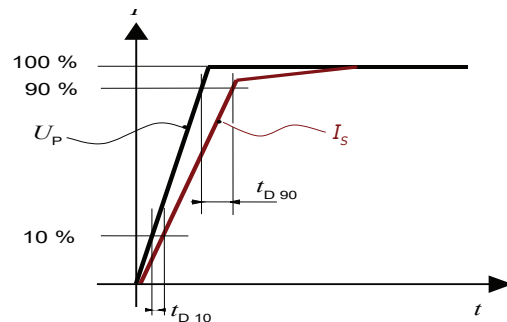
Figure 17: Delay time t_{D90} @ 90 and delay time t_{D10} @ 10
