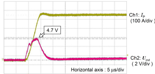
Example of Induced voltage: U_{ind} at the test winding I_p = 0 to 500 A at 5 \mu s ( di/dr = 100 A/ \mu s )
