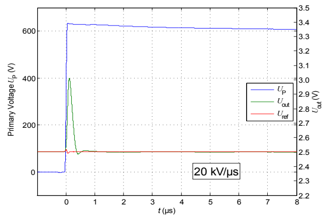
Figure 5: dV/dt
