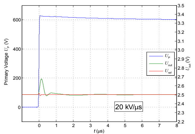
Figure 10: dv/dt
