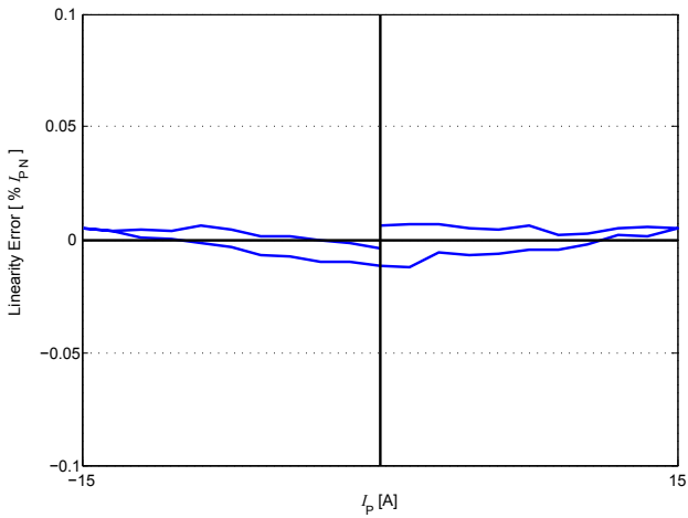
Figure 6: Linearity error
