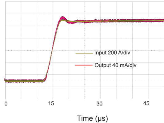
Figure 2: Typical step response (0 to 1 kA, 200 A/ \mu\text{s} )
