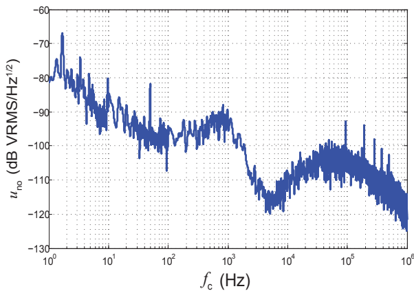
Figure 3: Typical output noise spectral density u_{no} with R_M = 100\ \Omega
