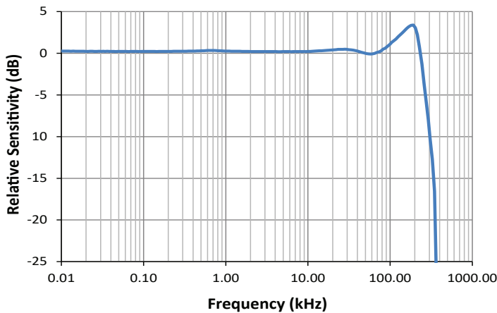
Figures 5 and 6: Typical frequency response, small signal bandwidth
