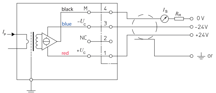
Figure 5: Connection principle
