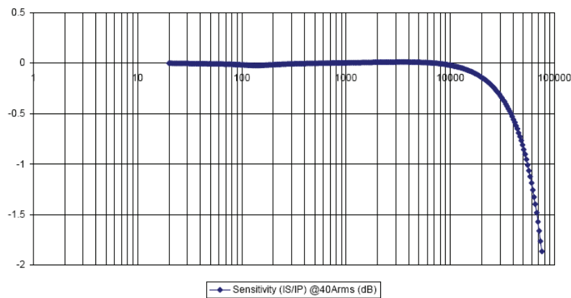
Figure 3: Bandwidth
