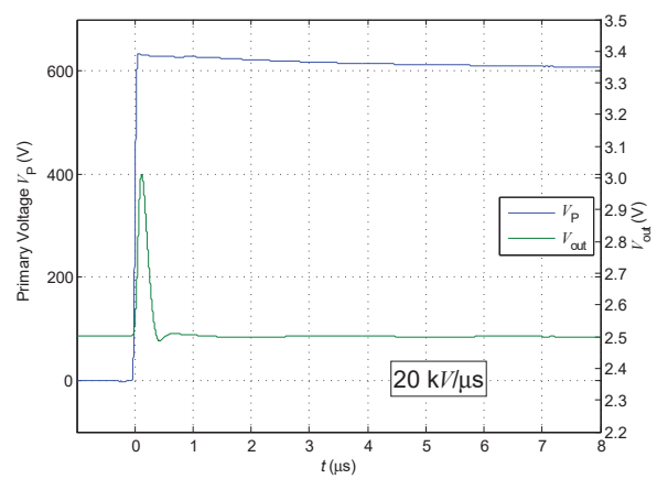
Figure 5: dv/dr
