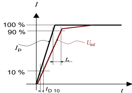
Figure 32: Delay time t_{D90} and reaction time t_{D10}
