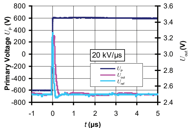
Figure 10: Step response
