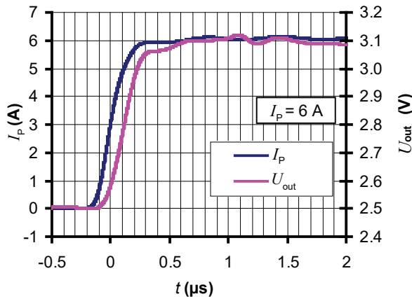
Figure 3: Step response
