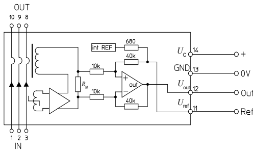
Figure 31: Test connection
