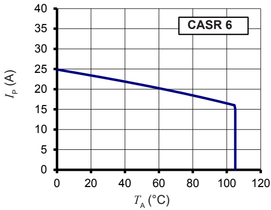
Figure 25: I_p vs T_A for CASR 6-NP/SP6
