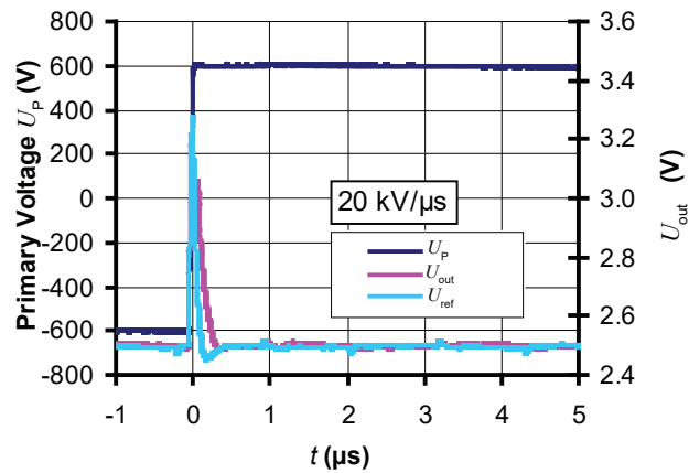
Figure 24: dv/dt
