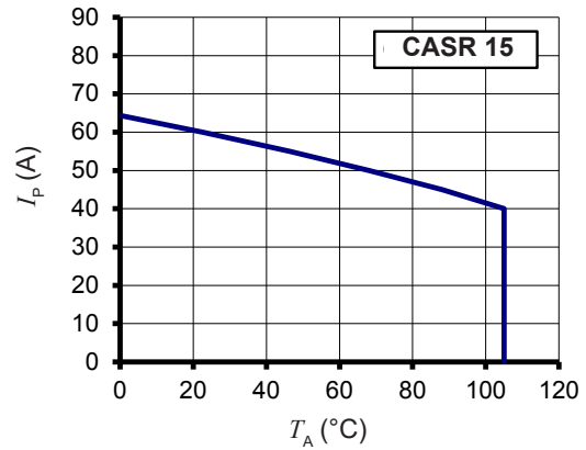
Figure 26: I_p vs T_A for CASR 15-NP/SP6
