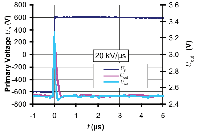
Figure 16: Step response
