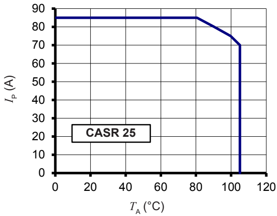
Figure 27: I_p vs T_A for CASR 25-NP/SP6
