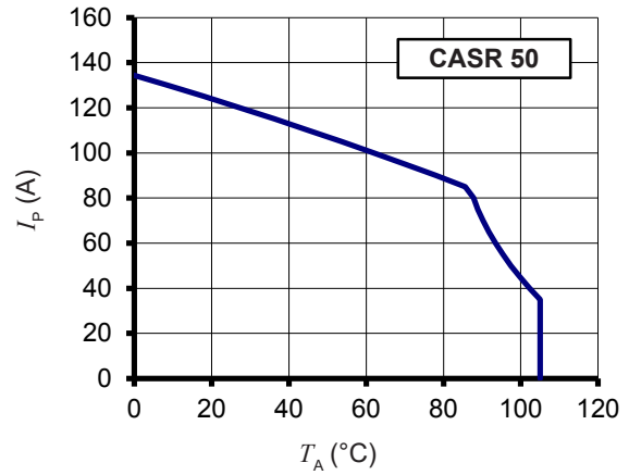
Figure 28: I_p vs T_A for CASR 50-NP/SP6
