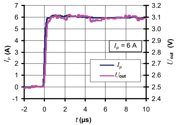
Figure 4: Step response
