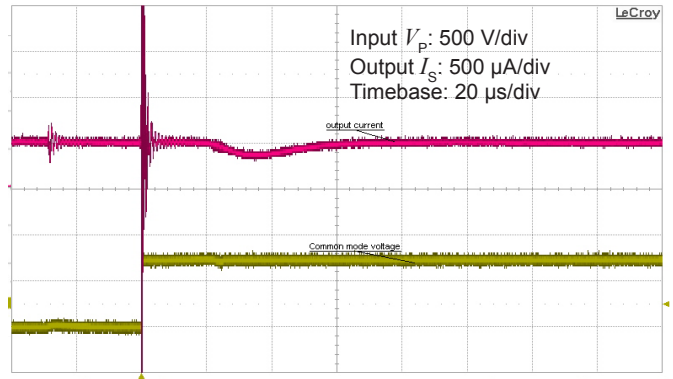
Figure 12: Detail of typical common mode perturbation (750 V step with 6 kV/μs, R_M = 100 \Omega )
