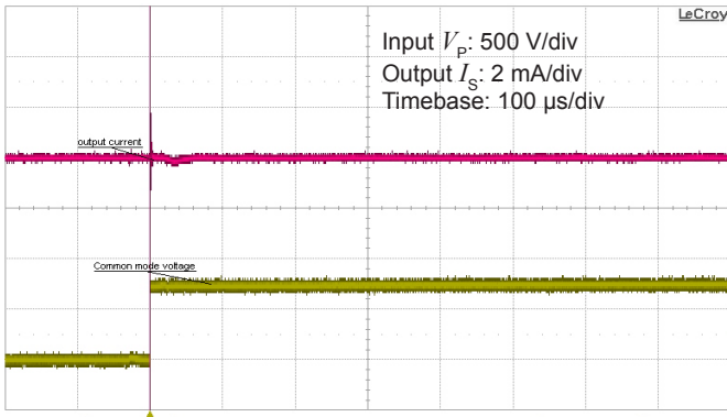
Figure 11: Typical common mode perturbation (750 V step with 6 kV/μs, R_M = 100 \Omega )
