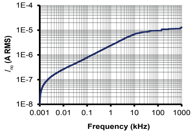
Figure 14: Typical total output RMS noise current with R_M = 50 \Omega
