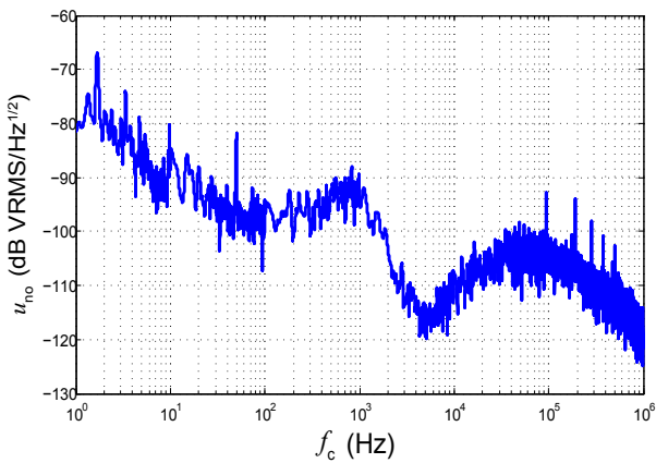
Figure 3: Noise voltage spectral density referred to primary u_{no} with R_M = 100 \Omega
