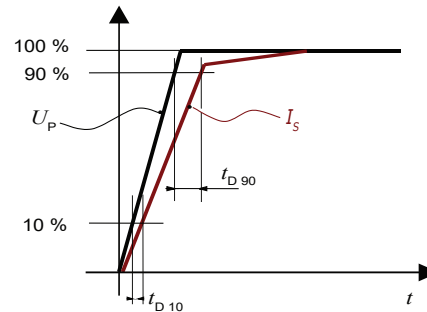
Figure 17: Delay time t_{D90} @ 90 and delay time t_{D10} @10
