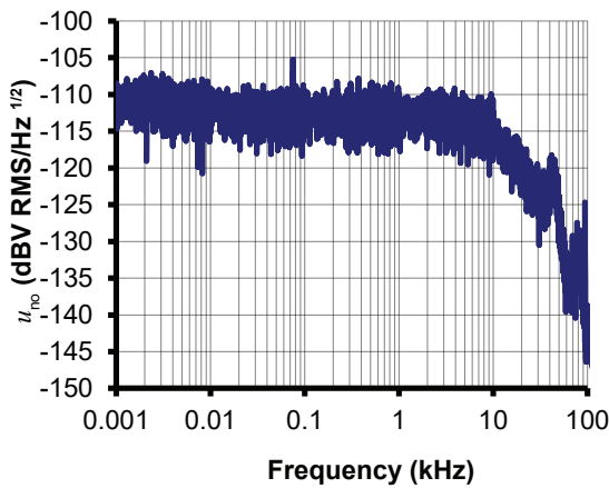
Figure 13: Typical noise voltage spectral density u_{no} with R_M = 50 \Omega
