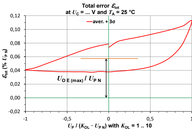
Figure 14: Total error \varepsilon_{tot}
