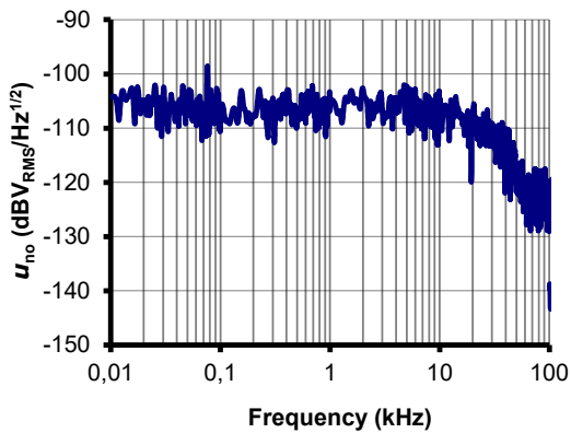
Figure 8: Typical output noise voltage spectral density u_{no} referred to secondary with R_M = 50 \Omega
