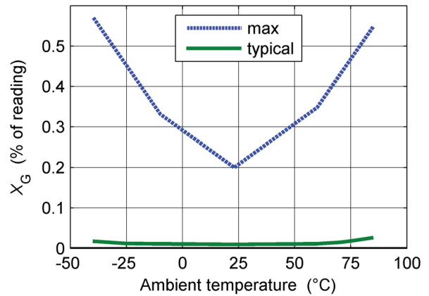
Figure 2: Overall accuracy in temperature for 0.1 I_{PN} \leq I_P \leq 1.5 I_{PN}
