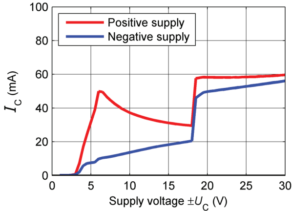
Figure 7: Typical supply current function of supply voltage ( I_p = 0 A )
