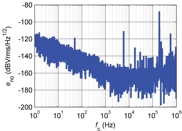
Figure 13: Typical noise voltage spectral density e_{no} with R_M = 1 \Omega
