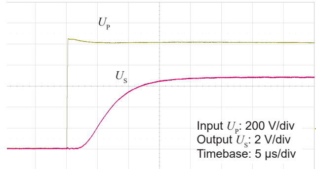
Figure 7: Typical step response (0 to 1000 V)
