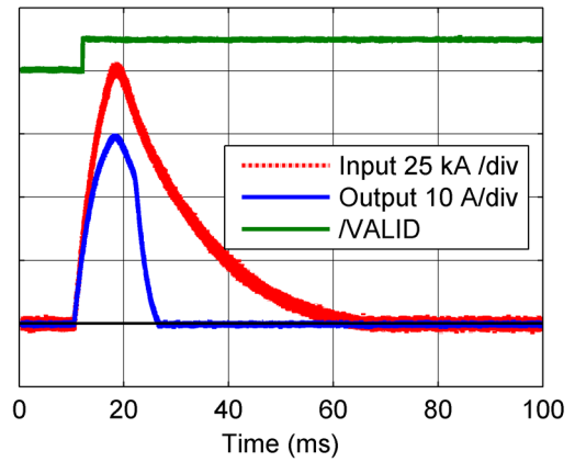
Figure 12: 100 kA overload behaviour
