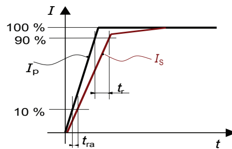
Figure 24: Response time t_r and reaction time t_{ra}
